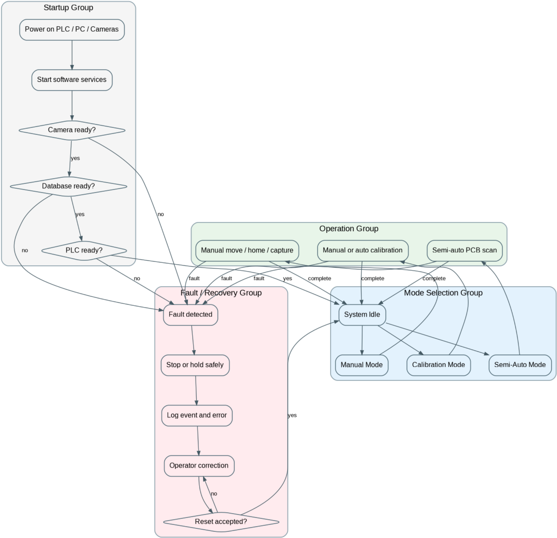
High-Level Control Flow Graph
