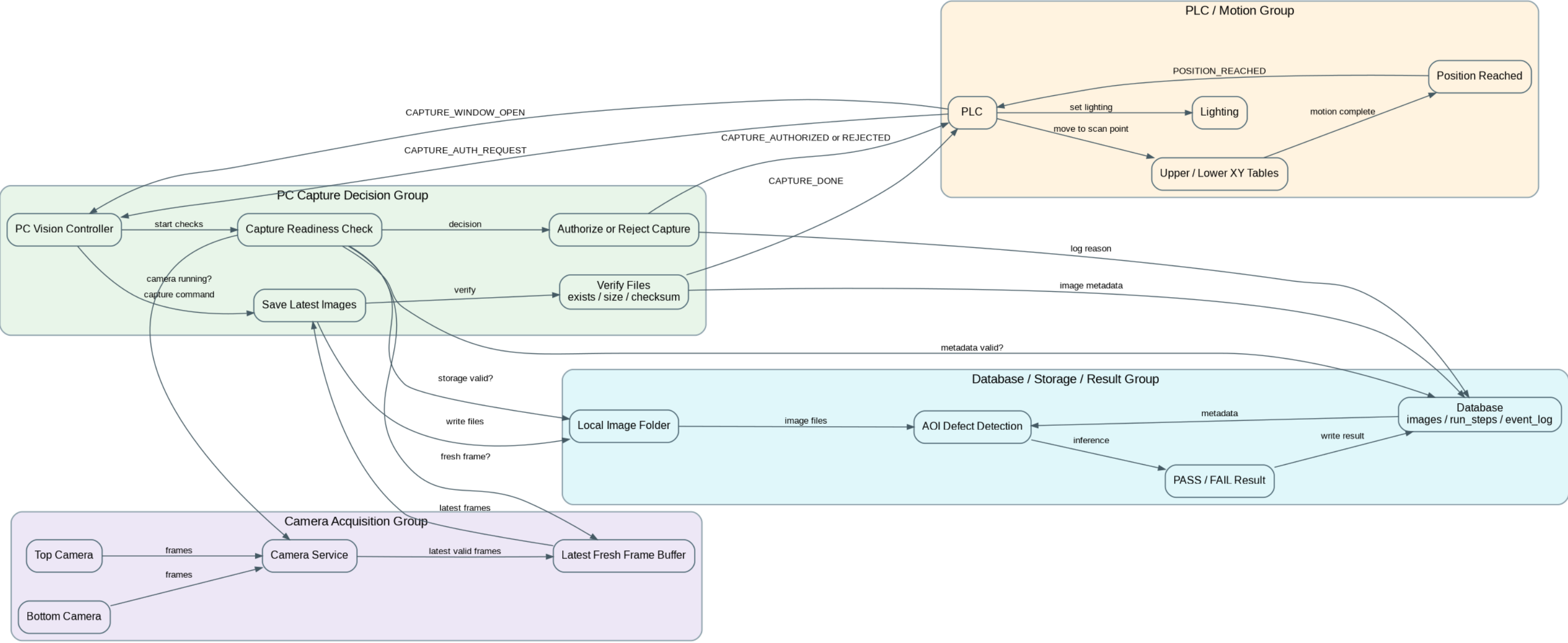
Vision Capture Dataflow Diagram
