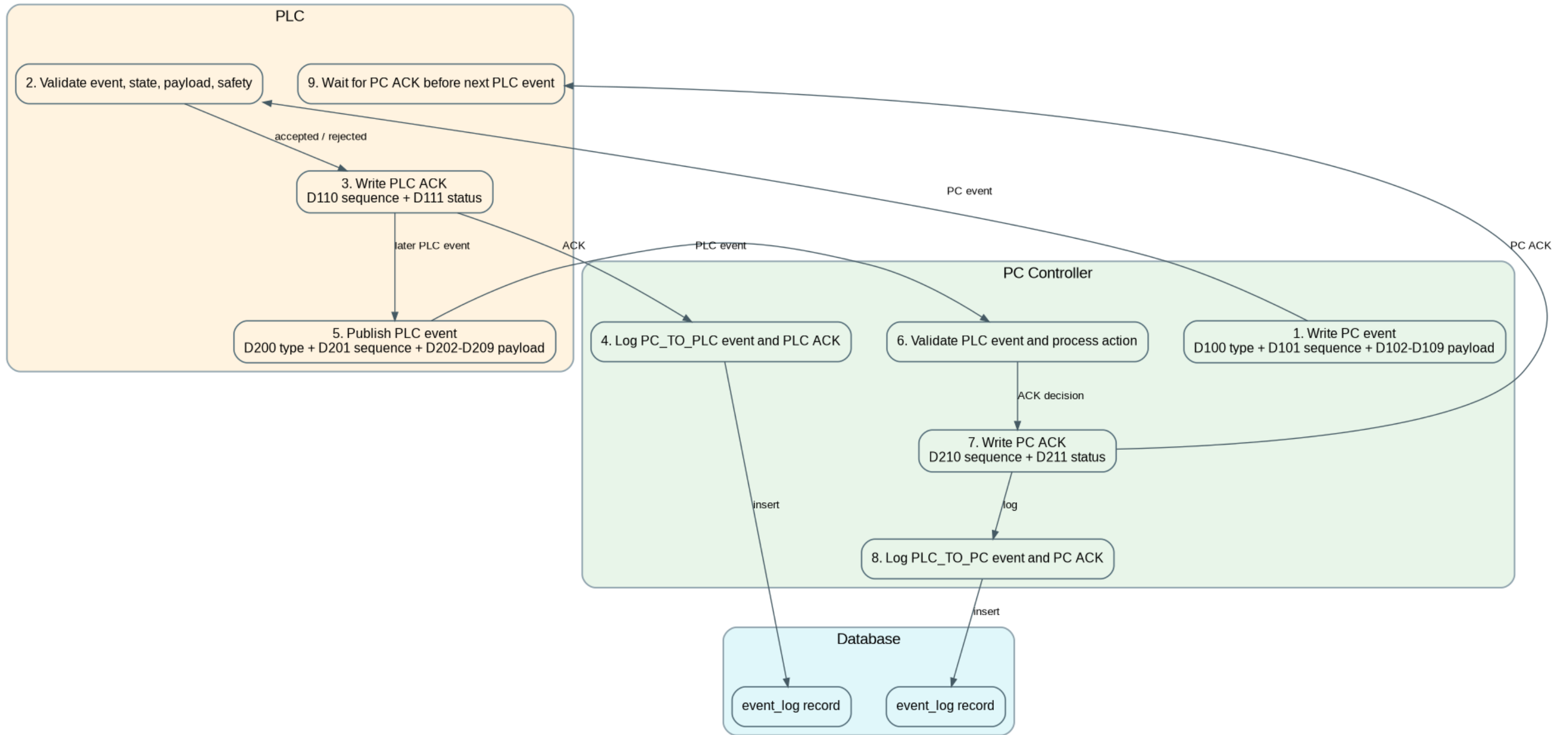
PC / PLC Event Communication Sequence
