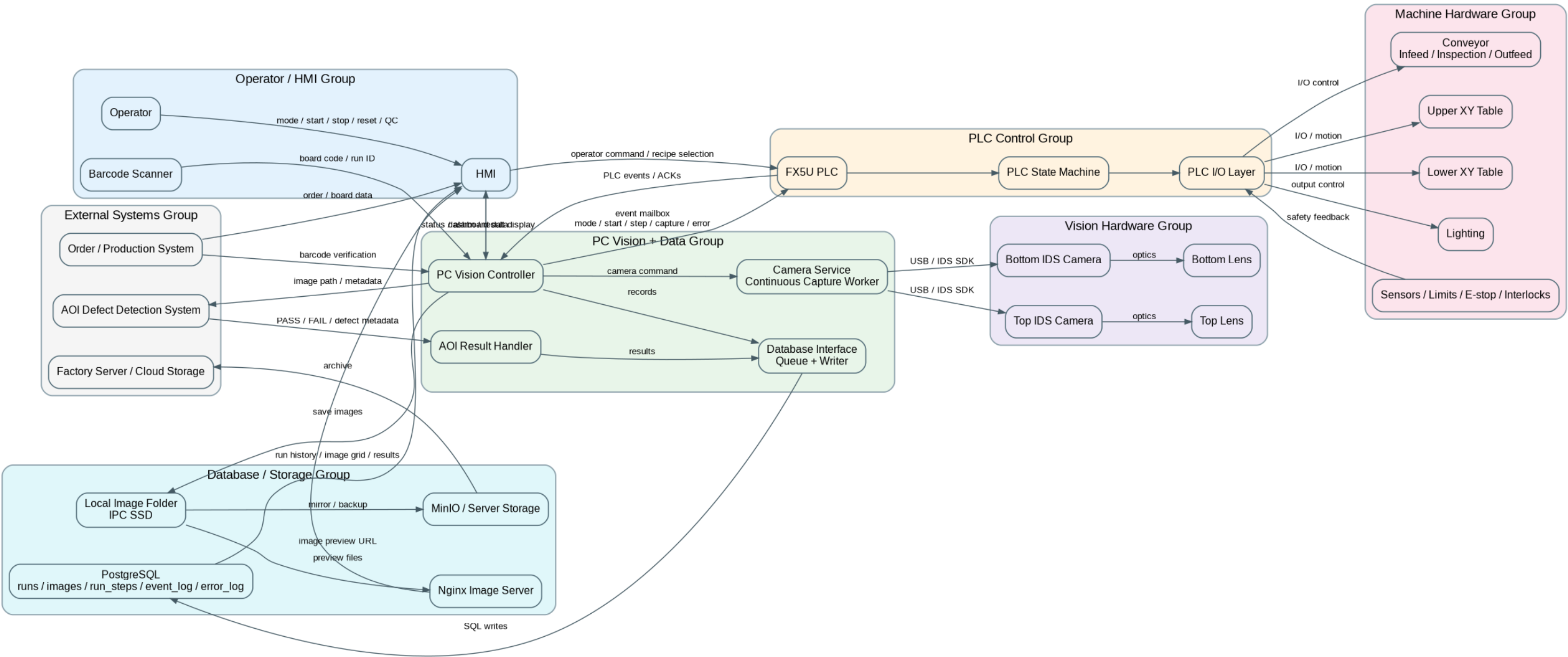
DUO_AOI Overall Functional Connection Diagram
